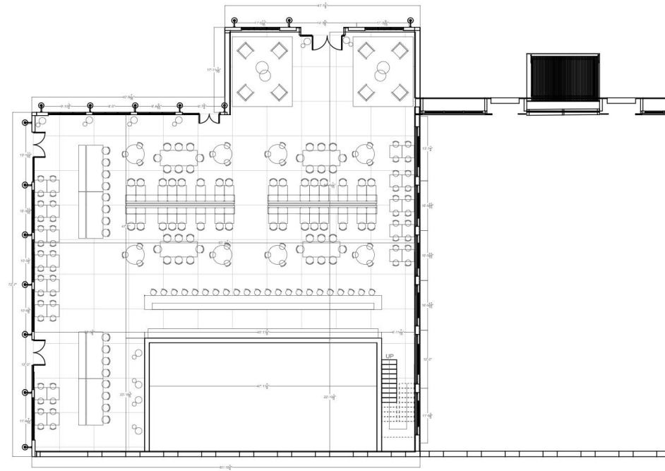
FIRST LEVEL
