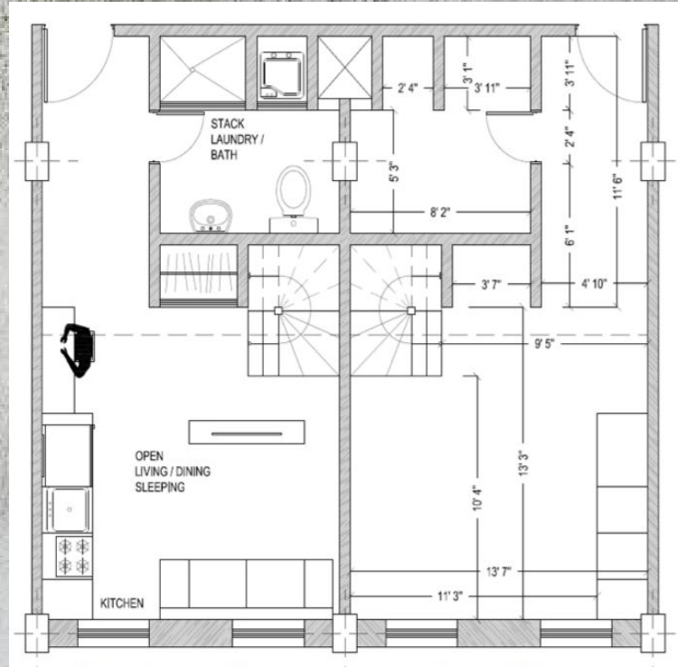
FURNITURE PLAN
