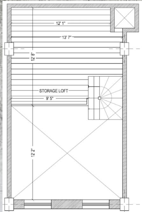
STORAGE LOFT PLAN
