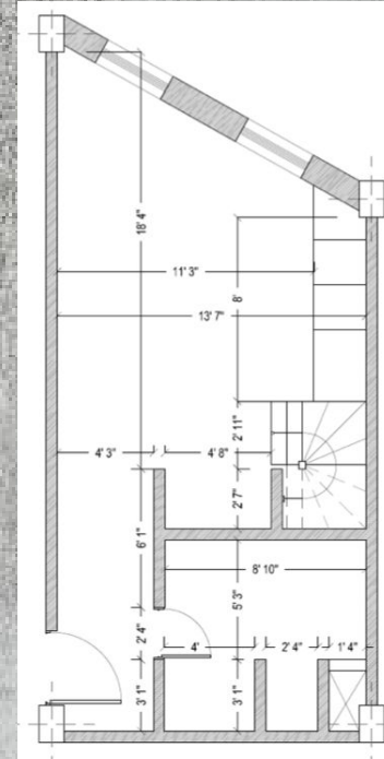
FLOOR PLAN
