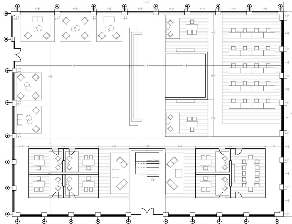
FIRST LEVEL
