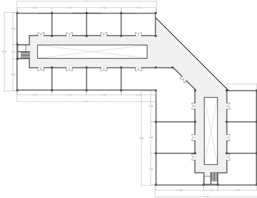
THIRD LEVEL
