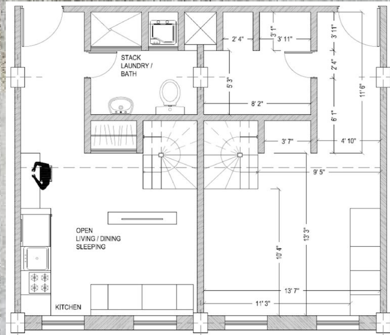
FURNITURE PLAN
