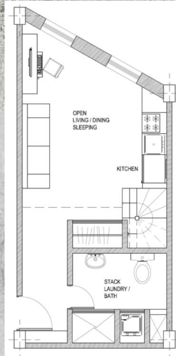
FURNITURE PLAN
